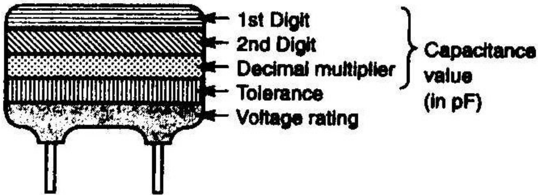
Polyester capacitor
